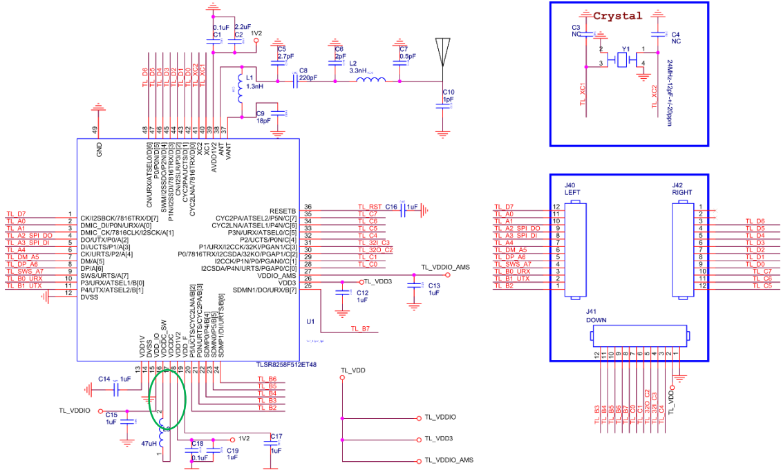
Figure 17- 1 Schematic
